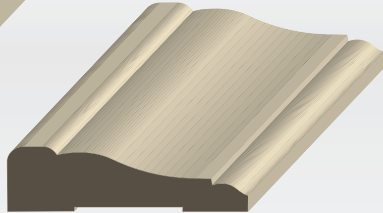
PX 20113 11/16" x 2-1/2"
